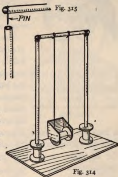
FIG. 314. — Doll Swing. FIG. 315. — Detail of Swing.
